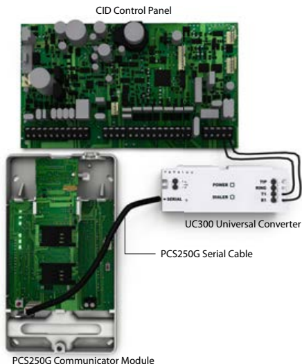
Figure 1: Connecting the PCS250G to an UC300
