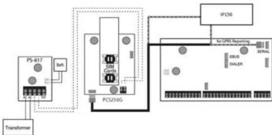
Figure 3: GPRS Serial Connections
