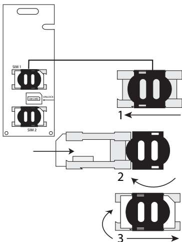
Figure 2: SIM Card Installation
