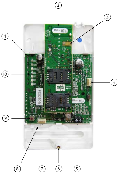
Figure 1: Inside the GPRS250G Module
