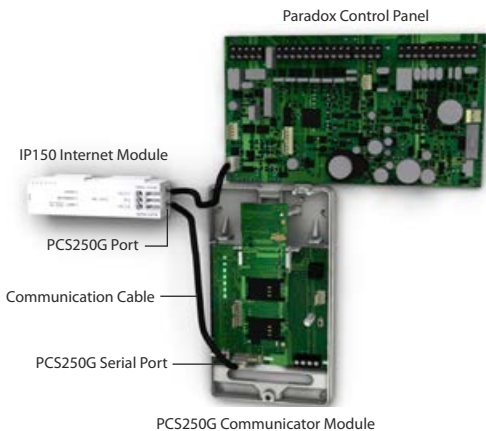
Figure 4: Interlinking Paradox Components
